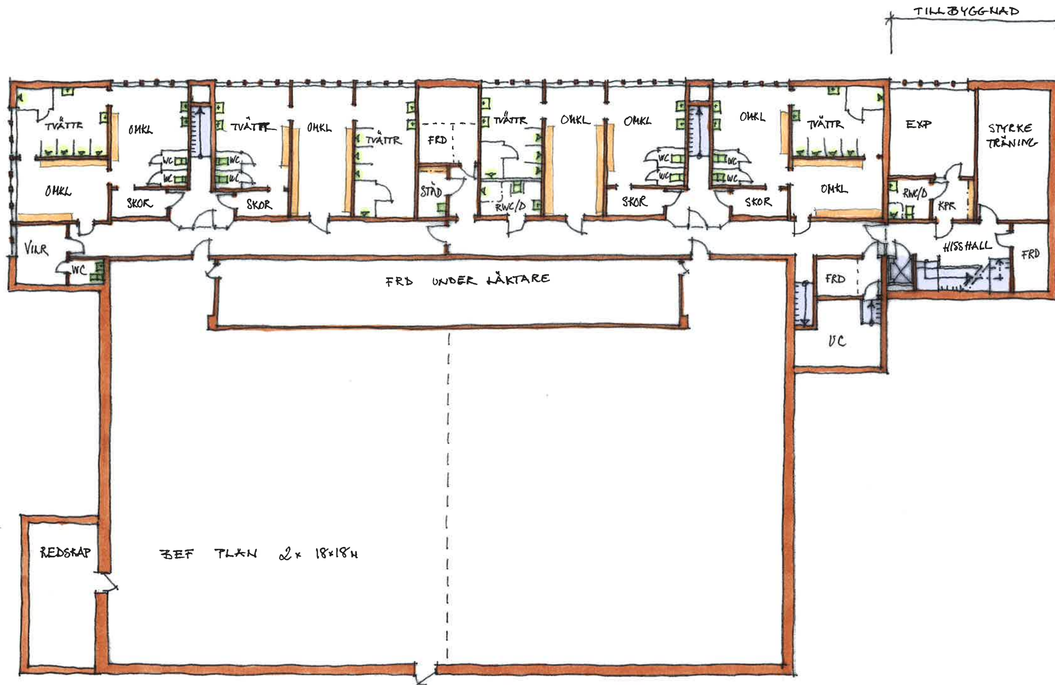
BOTTENPLAN
